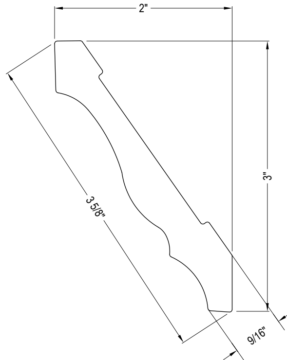
PROFILE
